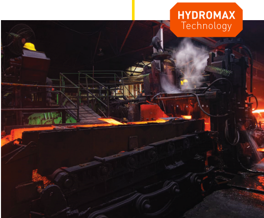
QUENCHING PROCESS WITH PATENTED ' HYDROMAX TECHNOLOGY '
